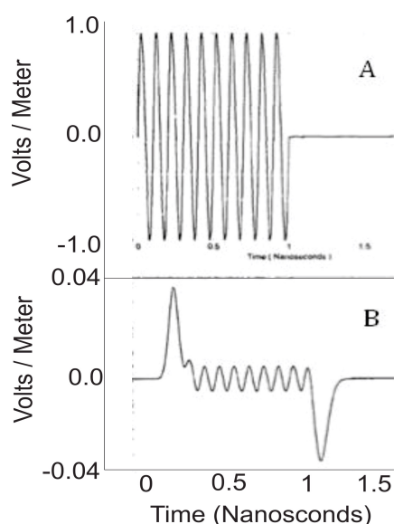
Figure 11: (After Albanese et al 1994) A: Injected pulse B: Same pulse after passage through 1 cm water
