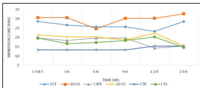
Figure 4. Inhibition zone diameters preexposure and postexposure to Wi-Fi radiation for Listeria monocytogenes .
