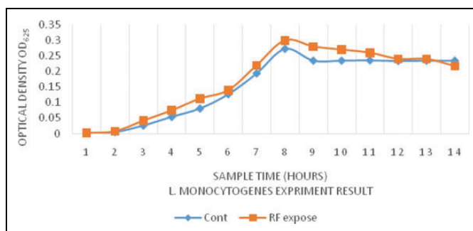
Figure 6. Growth curves Listeria monocytogenes in broth medium preexposure and postexposure.
